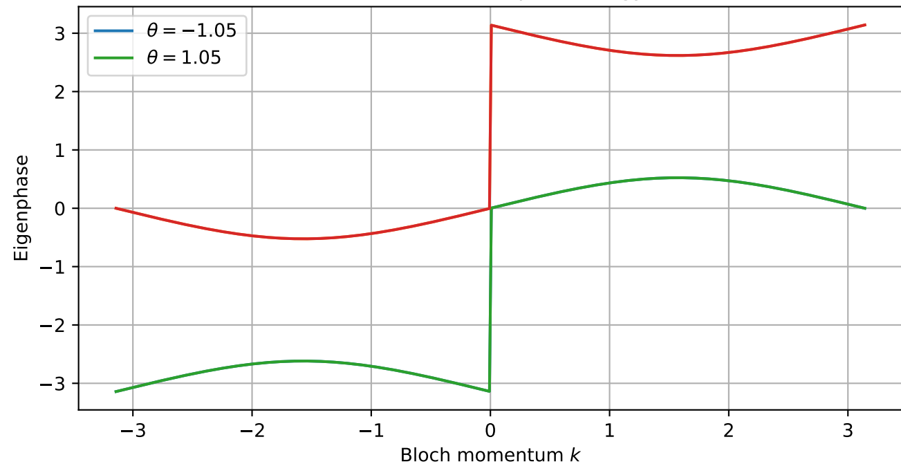
Periodic Eulerian walk quasienergy bands
