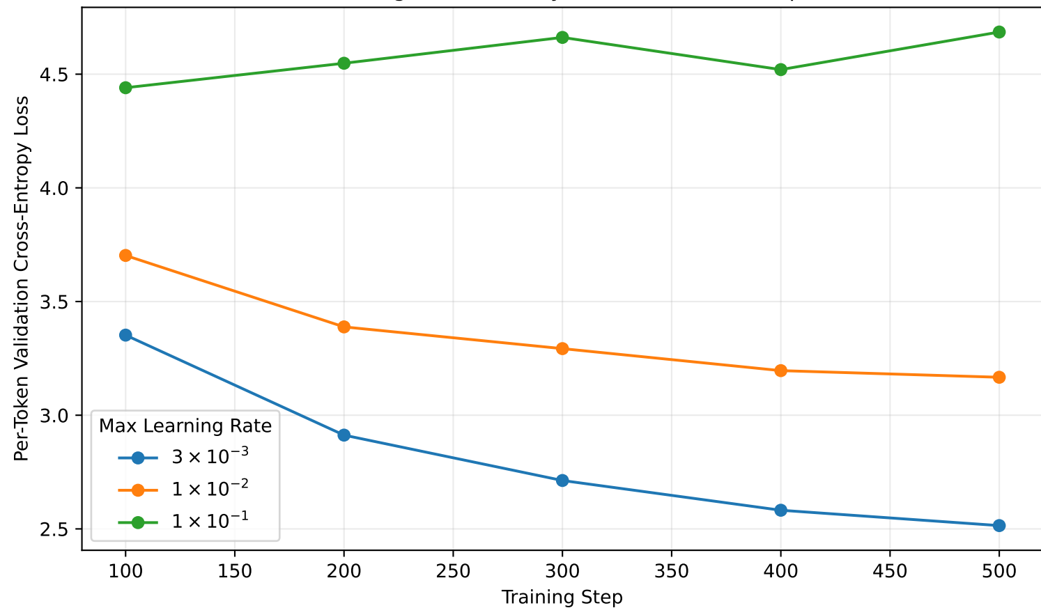
Learning Rate Stability Probe: First 500 Steps
