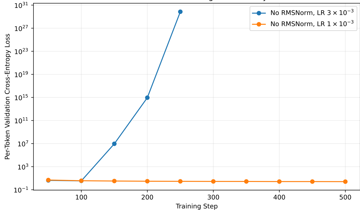
No-RMSNorm Learning Rate Stability
