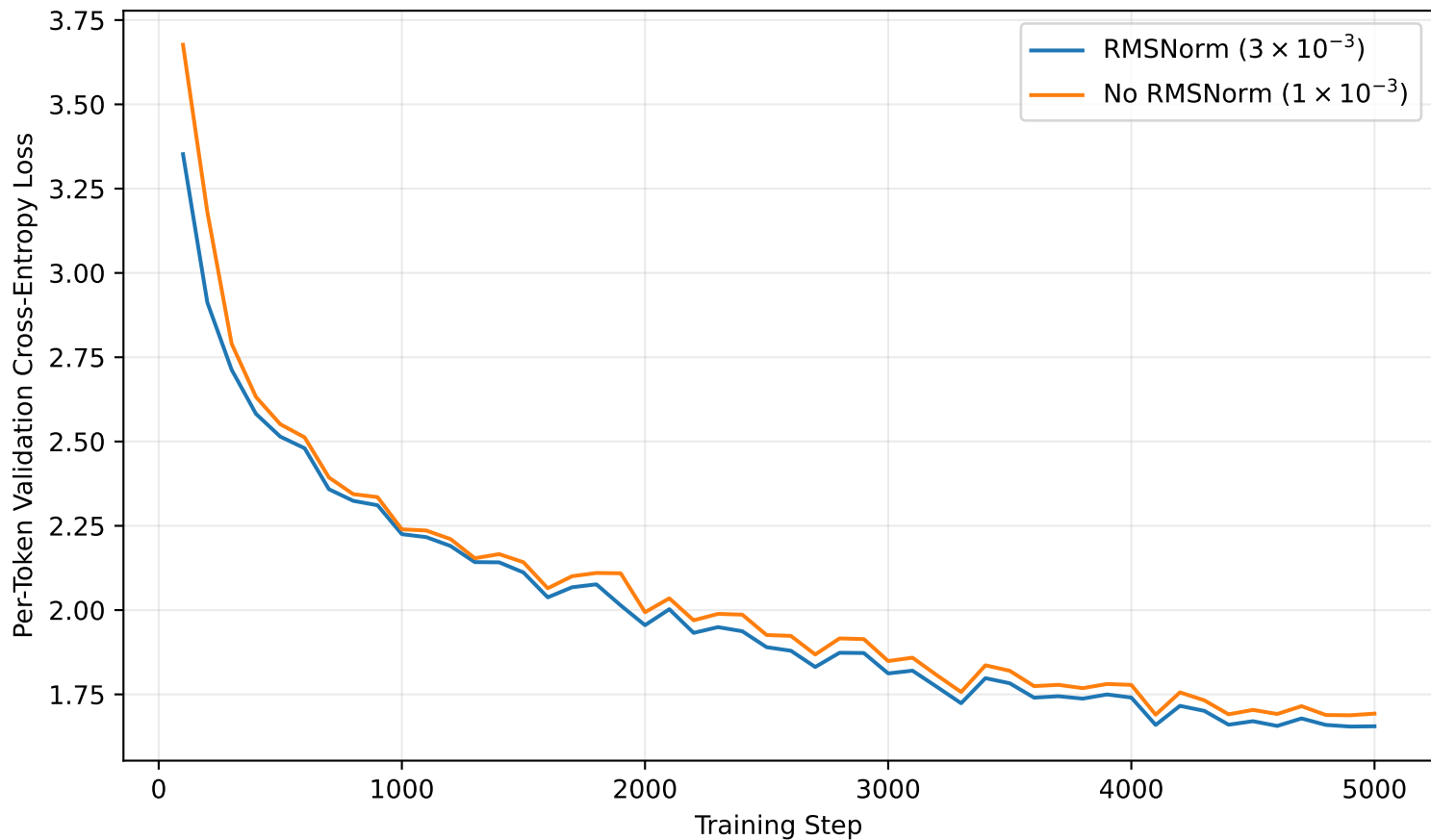
RMSNorm vs. No RMSNorm
