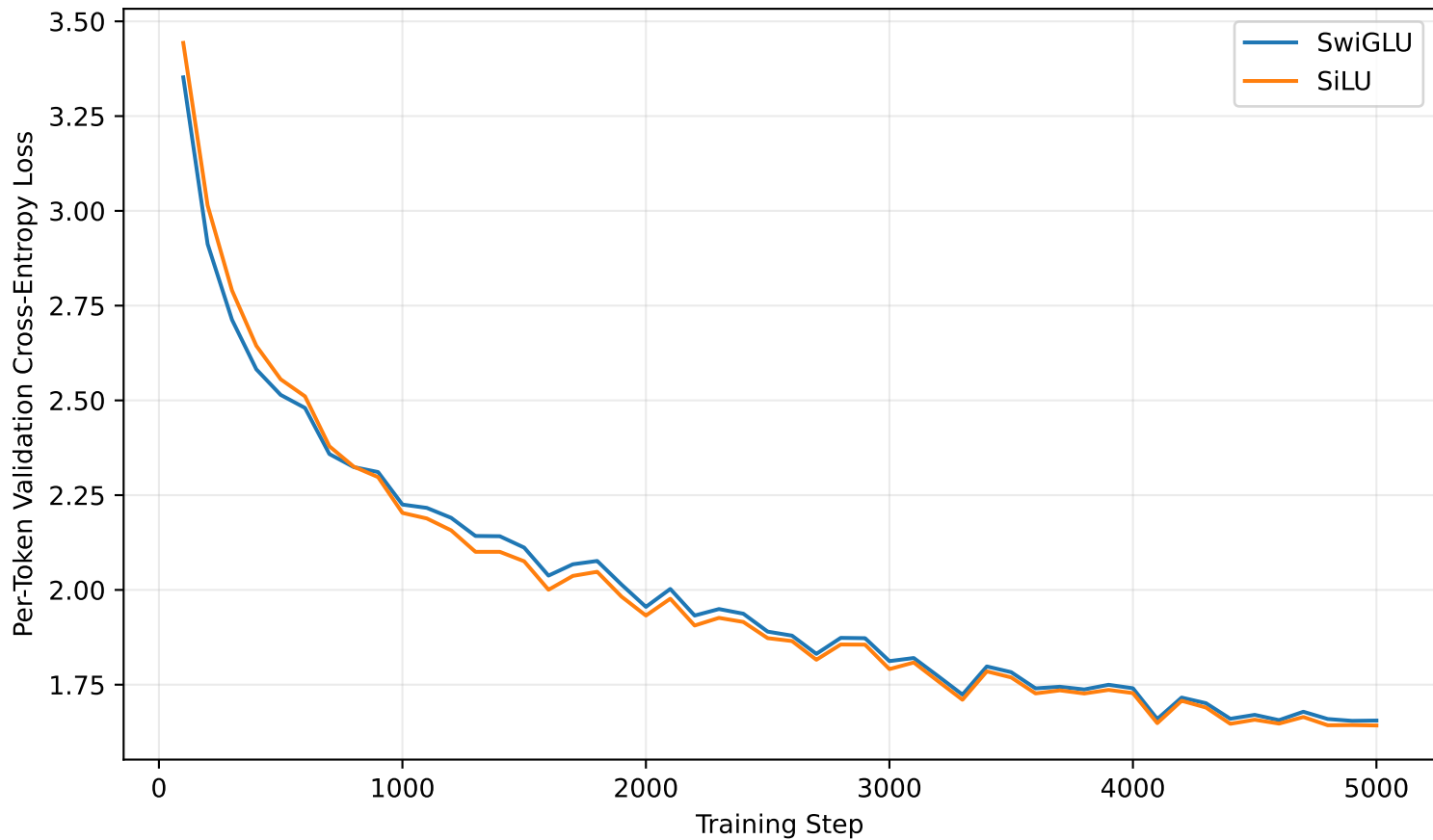
SwiGLU vs. SiLU
