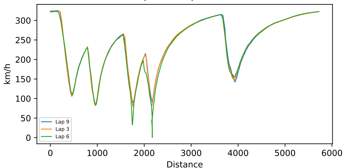
Speed over lap distance
