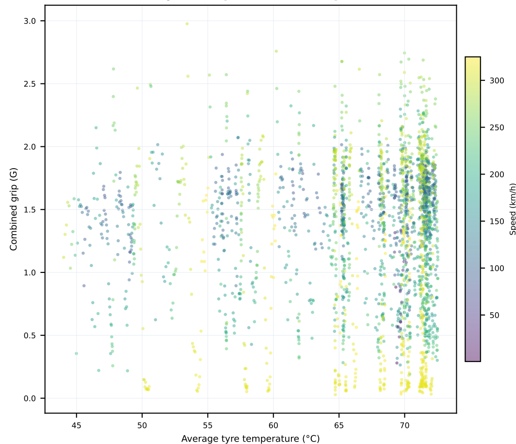
Tyre Temperature vs Grip
