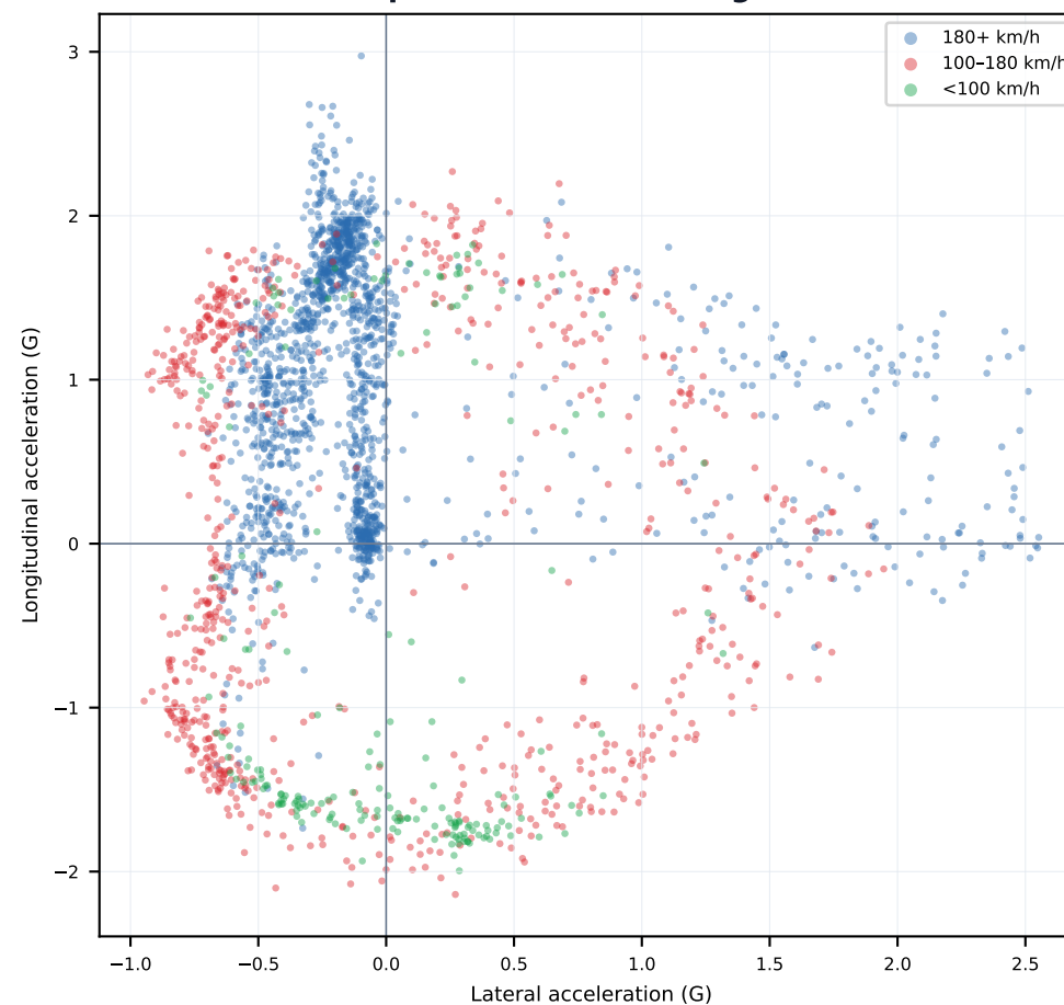
Speed-Binned G-G Diagram
