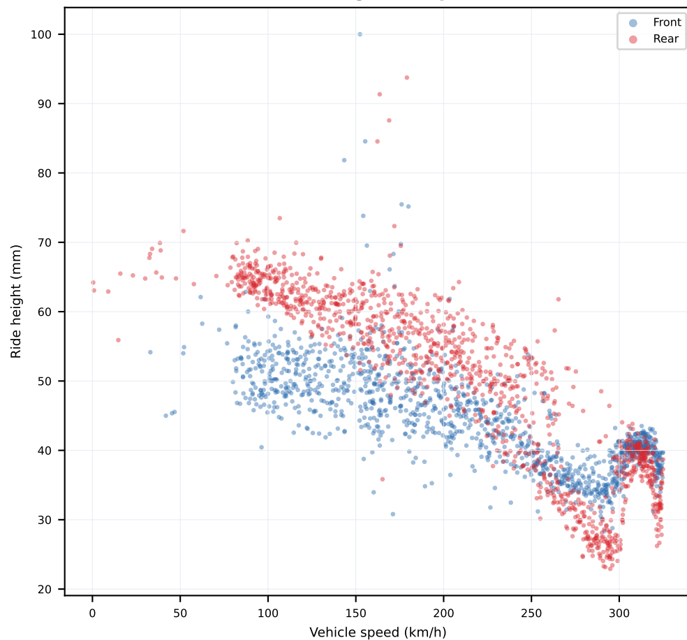
Ride Height vs Speed
