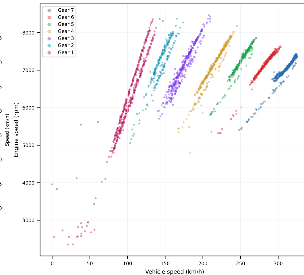
Gear Chart
