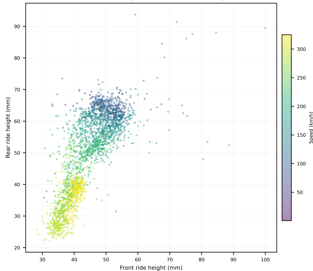
Front Ride Height vs Rear Ride Height
