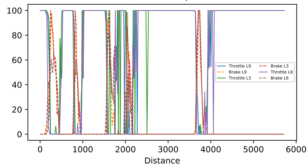
Throttle / brake over lap distance
