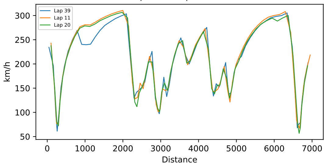
Speed over lap distance
