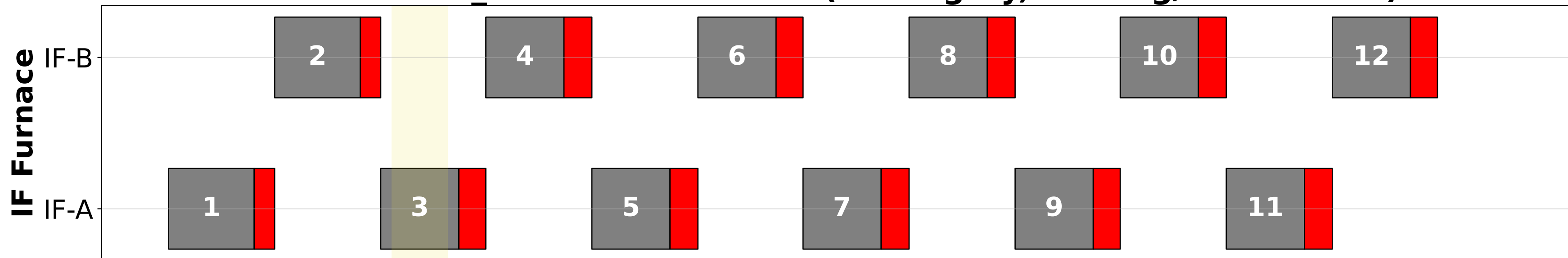
continuous_baseline - IF Gantt (melt=gray, holding/reheat=red)
