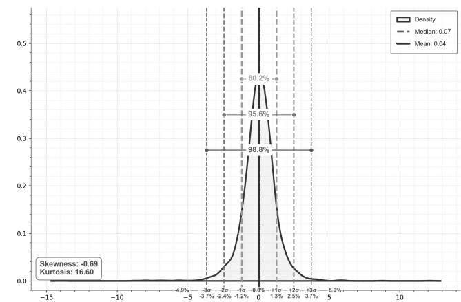
Density Plot Nifty 50 (10 Years, Monthly returns)
