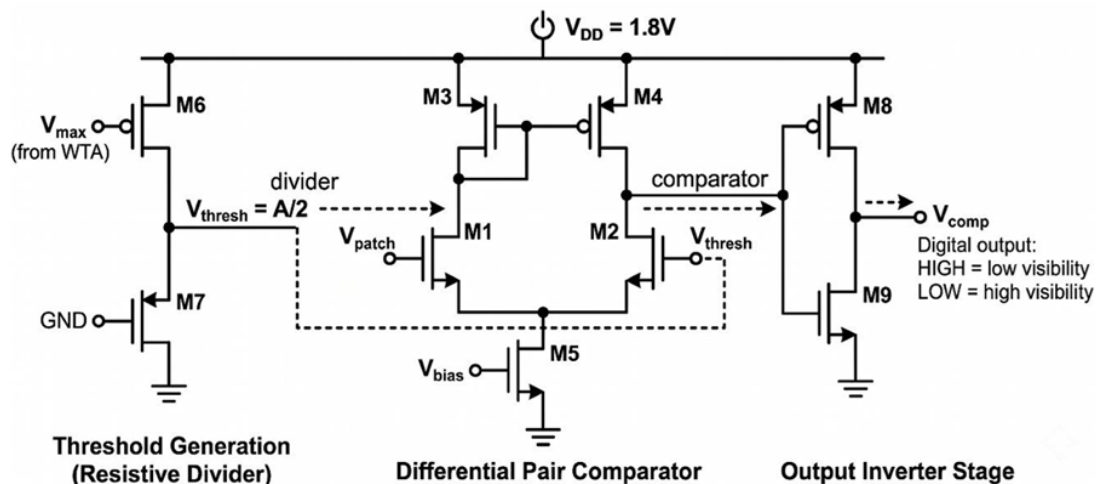
Figure 2: Circuit Diagram
