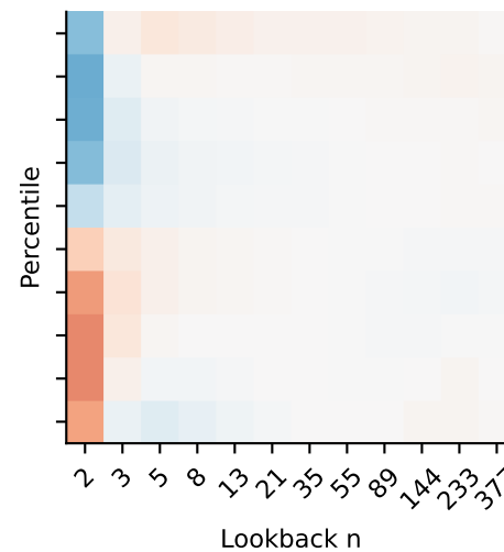
Student-t8
