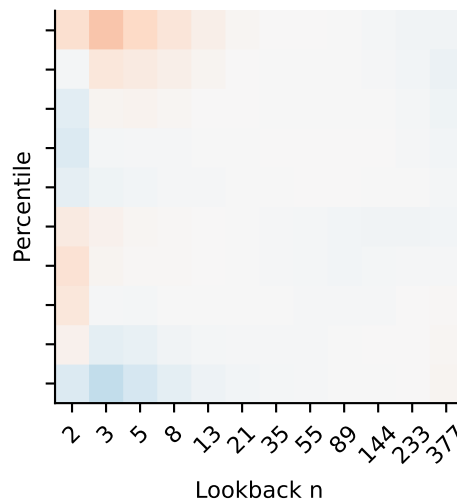
Student-t6
