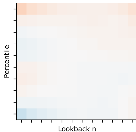
Laplace
