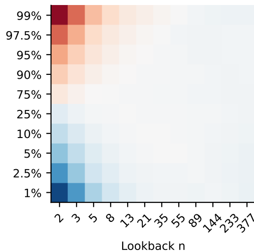
Student-t5
