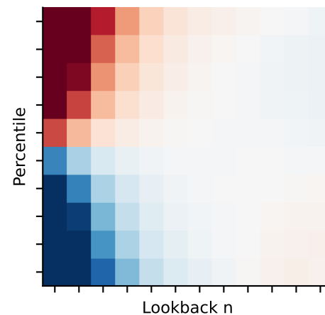
Student-t4
