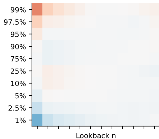
Gaussian
