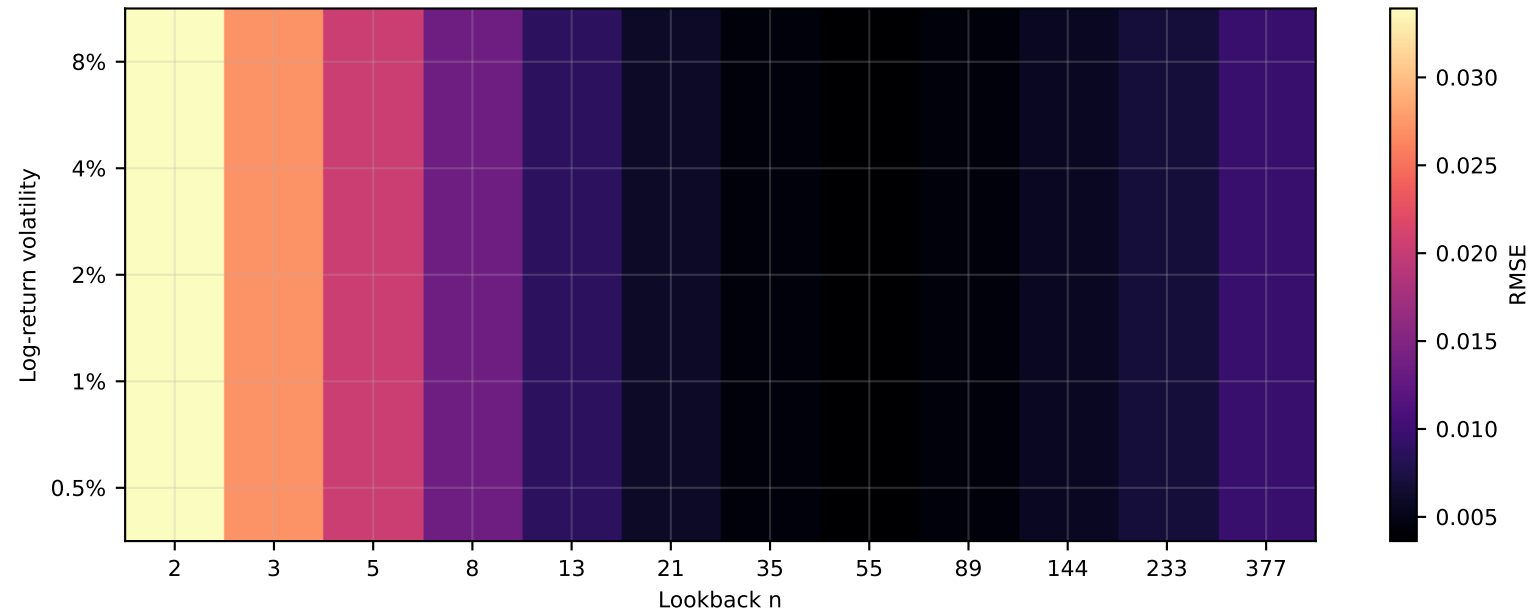
Quantile RMSE: Gaussian, log price
