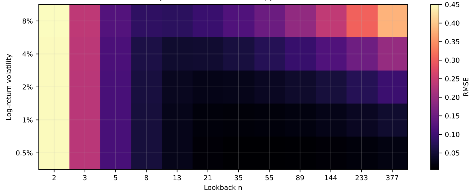
Quantile RMSE: Student-t4, price
