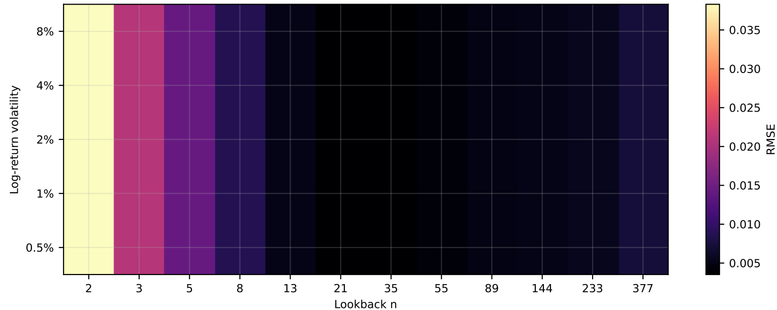
Quantile RMSE: Student-t6, log price
