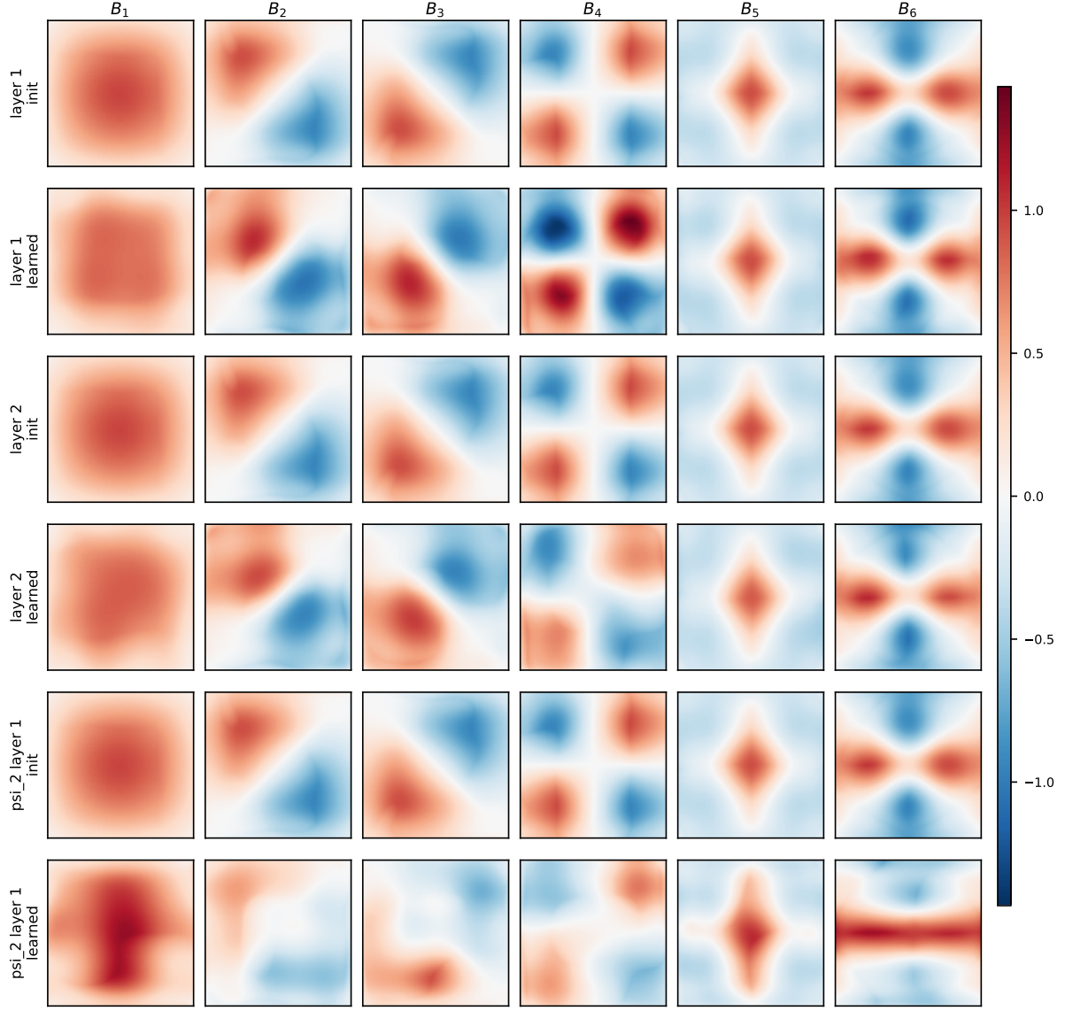
Figure 1: Learned multivariate rational basis functions of the PascalVOC model mv_K6 ( K = 6 , degrees (8, 6) , PCA-of-hats initialization, seed 0) on the pseudo-coordinate square [0, 1]^2 (Cartesian edge attributes, (0.5, 0.5) = \text{zero offset} ). Rows alternate between the initialization (the six leading principal components of the 5 \times 5 B-spline hats) and the functions after 15 epochs, for both layers of \psi_1 and the first layer of \psi_2 . The learned functions keep the overall layout of their initialization but sharpen and shift their extrema and develop asymmetric side lobes; the \psi_2 layer, which operates on the consensus features, moves furthest from its initialization. Figures for the hat-initialized K = 9 basis and for K = 4 are in paper/figures/(experiments/plot_basis.py) .
