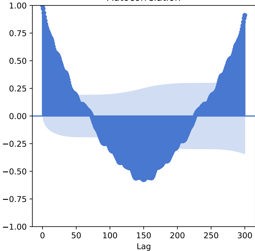
Autocorrelation
