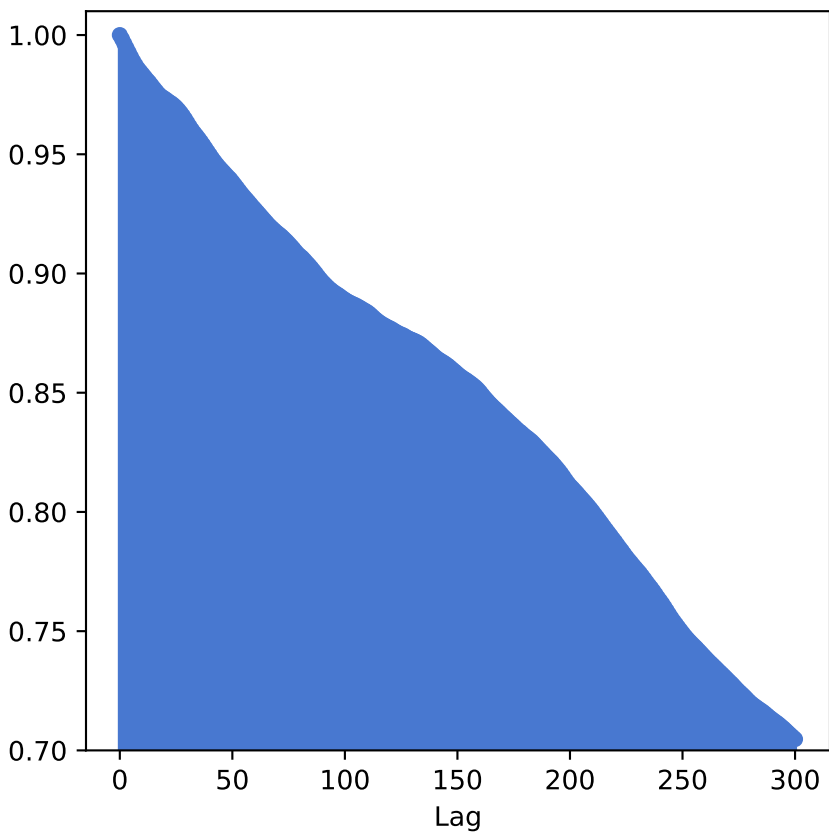
Autocorrelation
