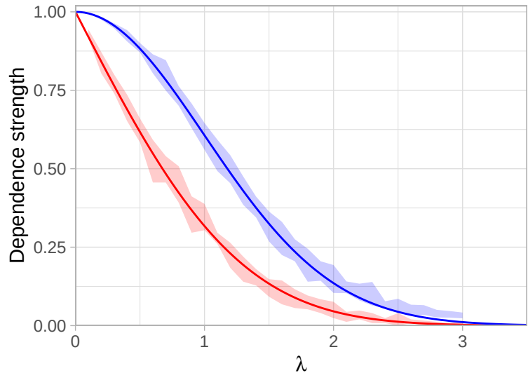
Hüsler-Reiss
