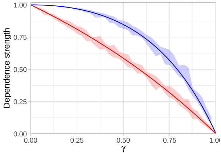
Symmetric logistic
