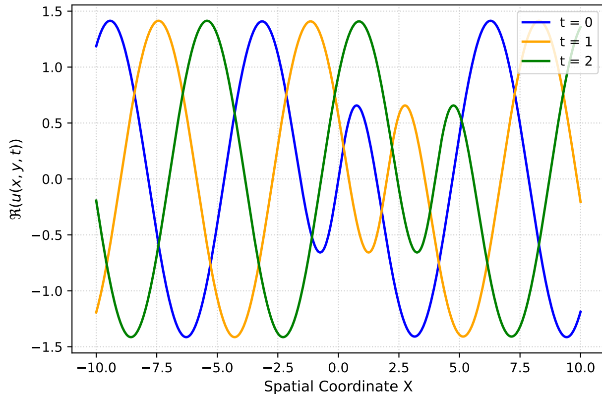
Real Part \Re(u) of the Dark Soliton
