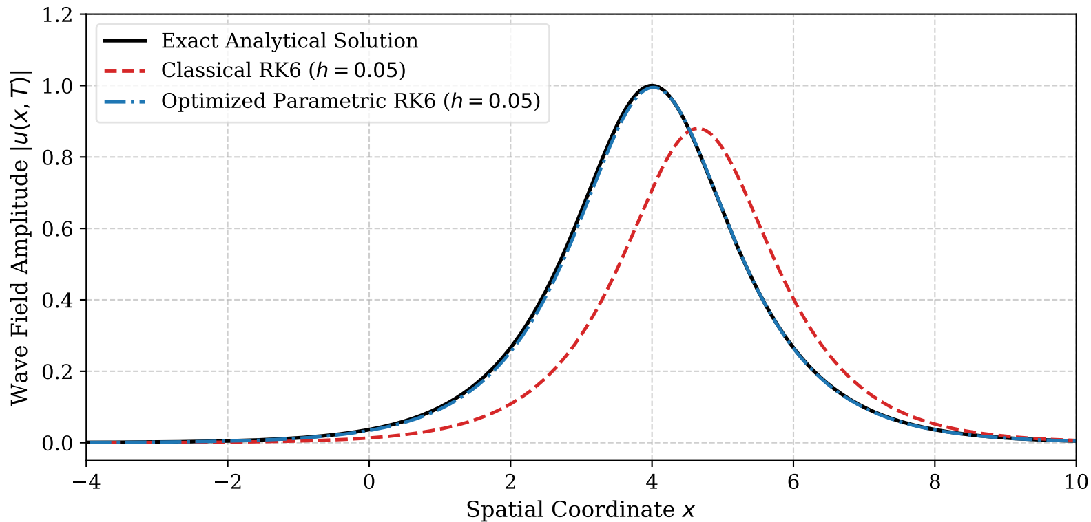
Soliton Profile Comparison at Final Time T = 2.0
