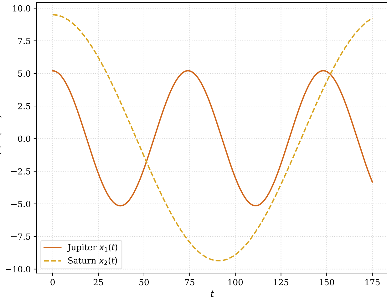
Time Domain: Selected Coordinate Oscillations
