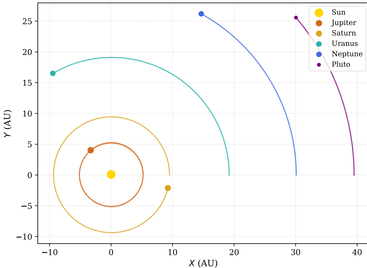
Space Domain: Concentric Planetary Orbits
