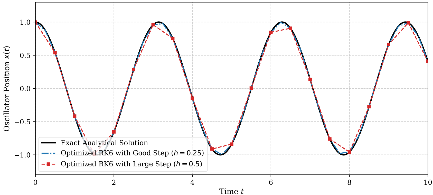
Linear Harmonic Oscillator: Step Size Error Accumulation
