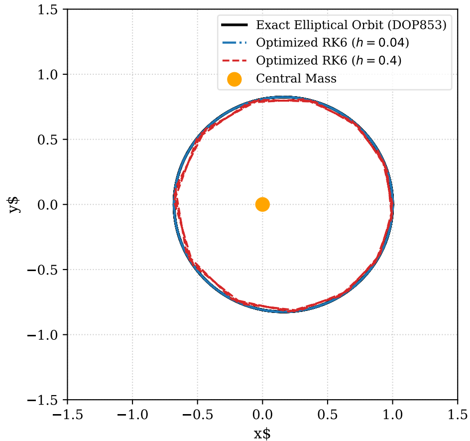
Space Domain: Trajectory Orbit Stability
