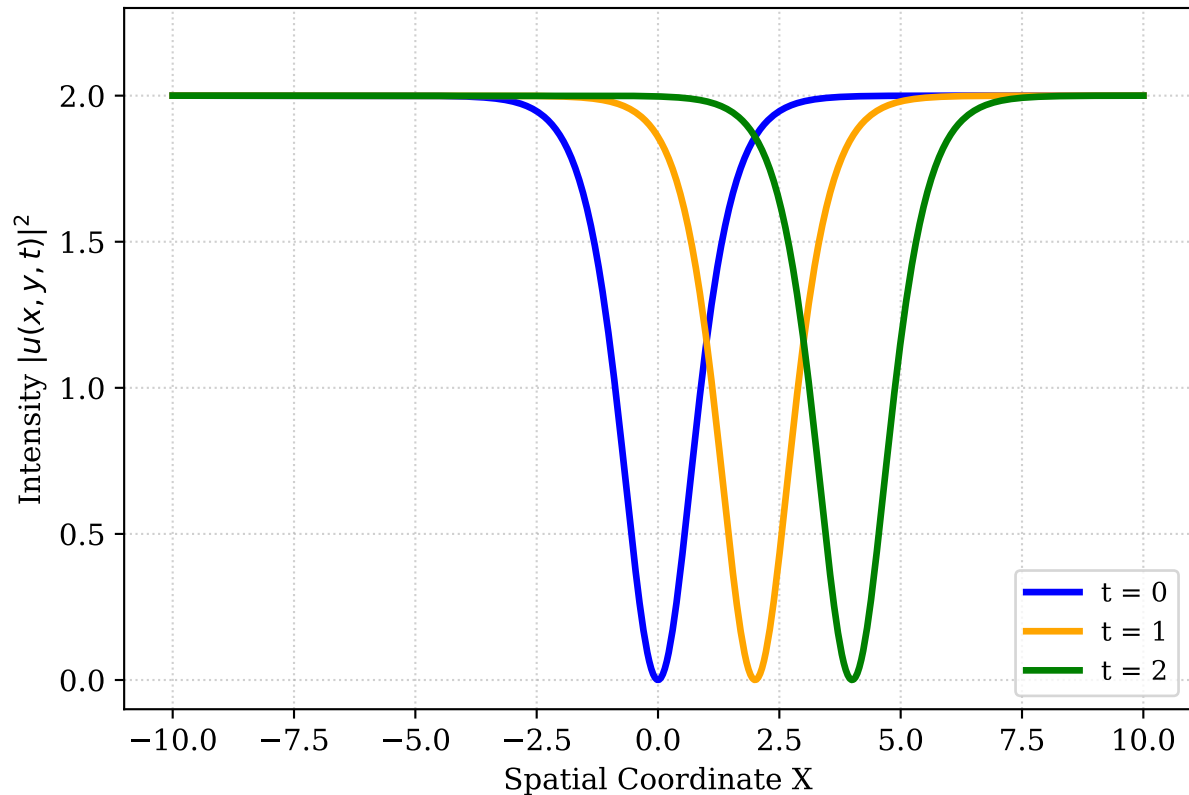
Dark Soliton Intensity Profiles over Time
