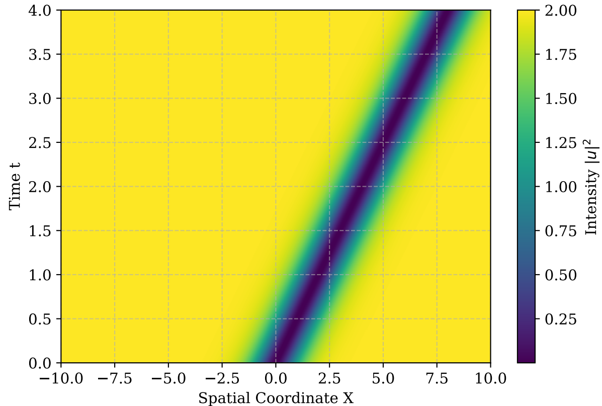
Spatiotemporal Evolution of Dark Soliton
