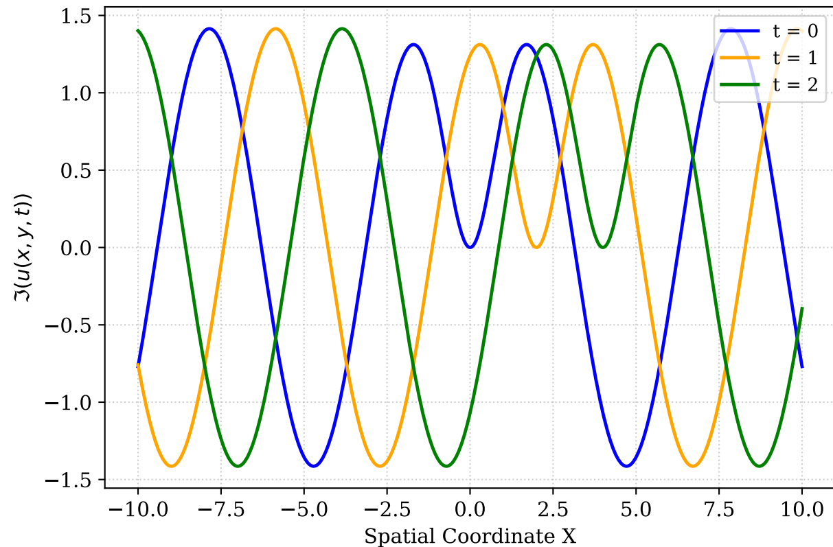
Imaginary Part \Im(u) of the Dark Soliton
