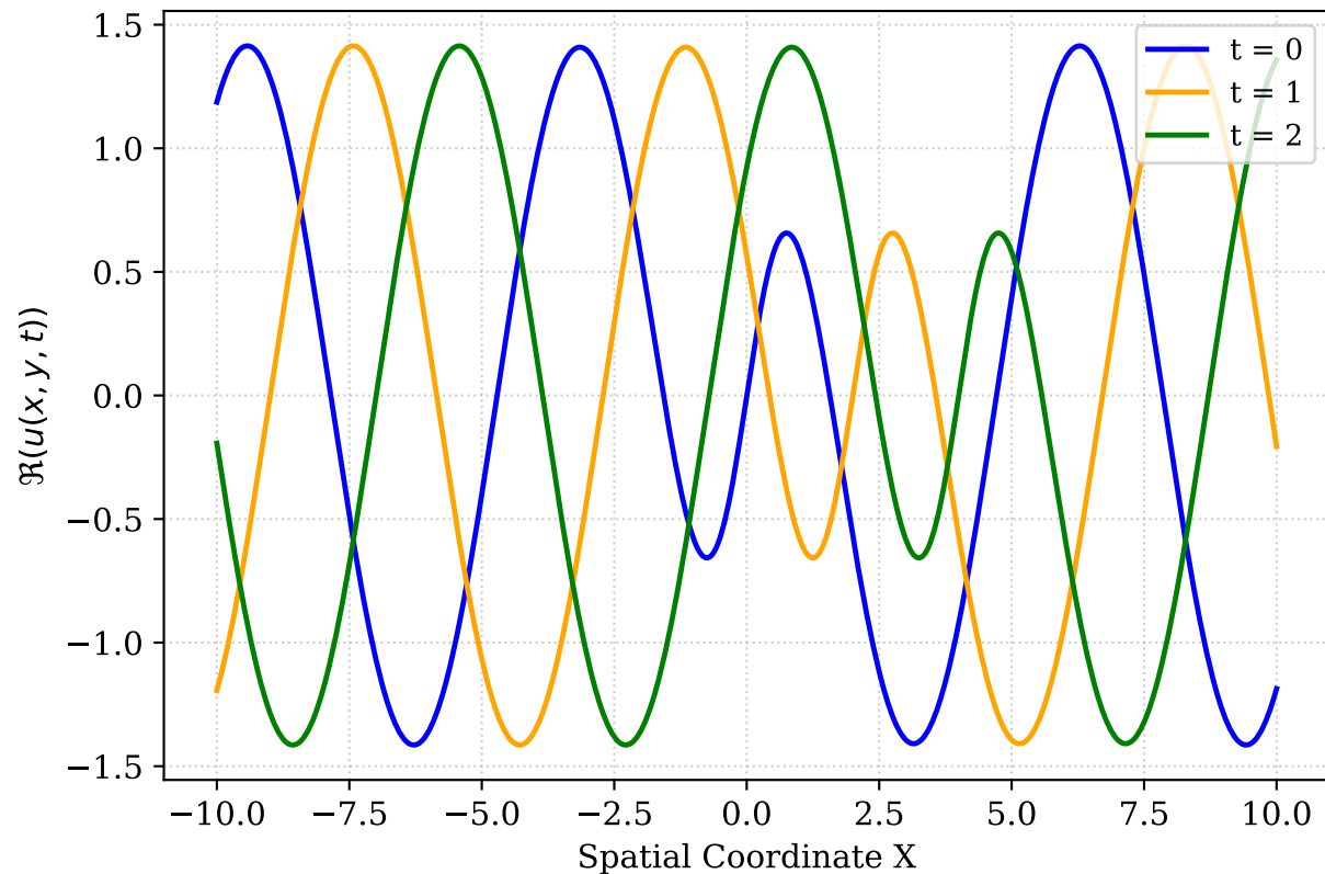
Real Part \Re(u) of the Dark Soliton
