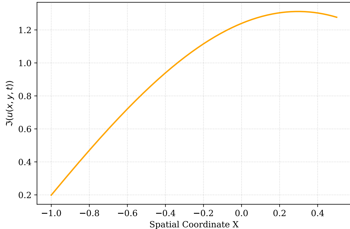
Imaginary Part \Im(u) of the Dark Soliton
