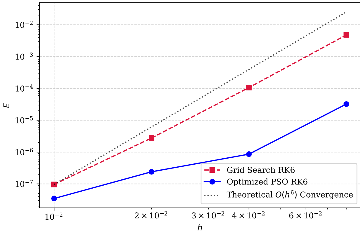
2D NLS Empirical Convergence Rate Verification
