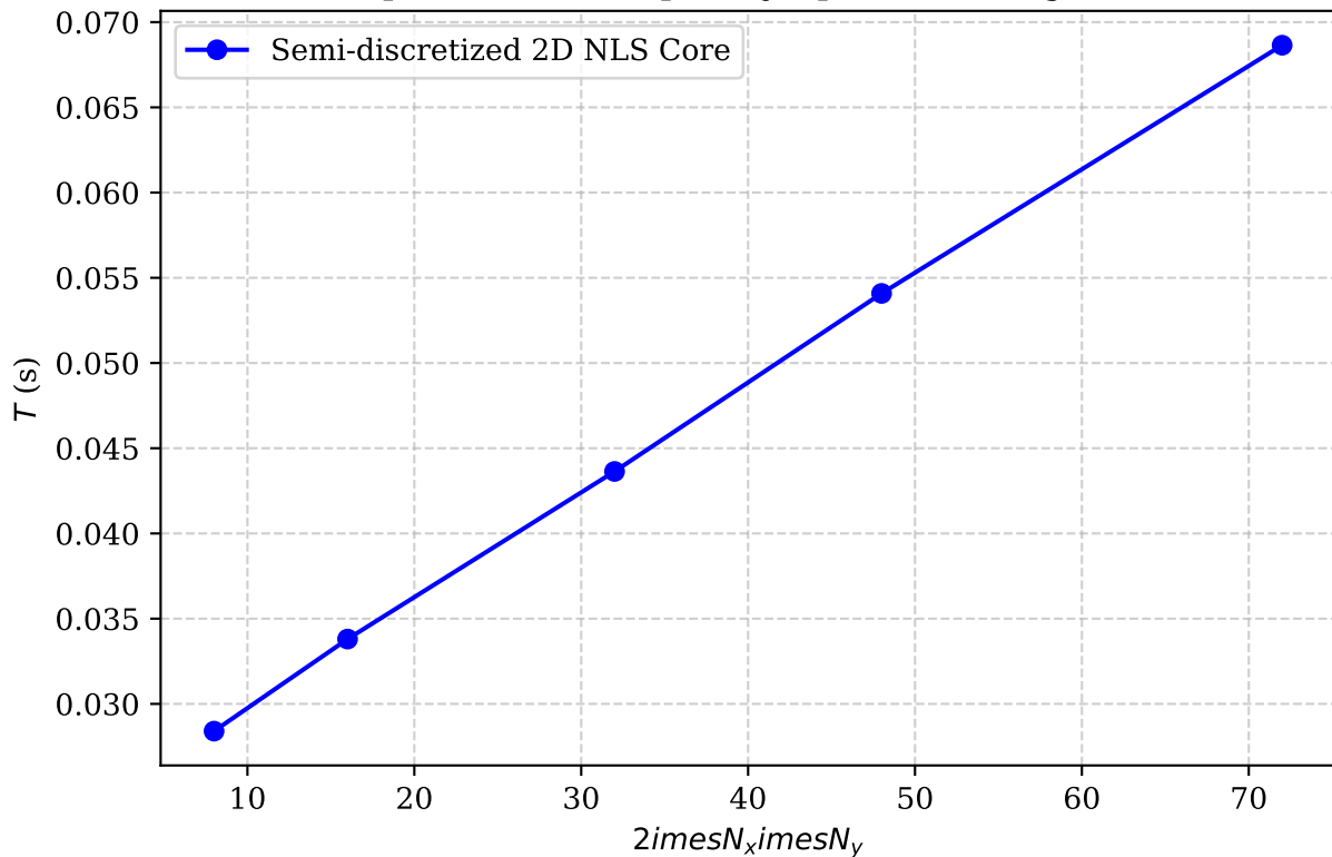
Computational Complexity Spatial Scaling Profile
