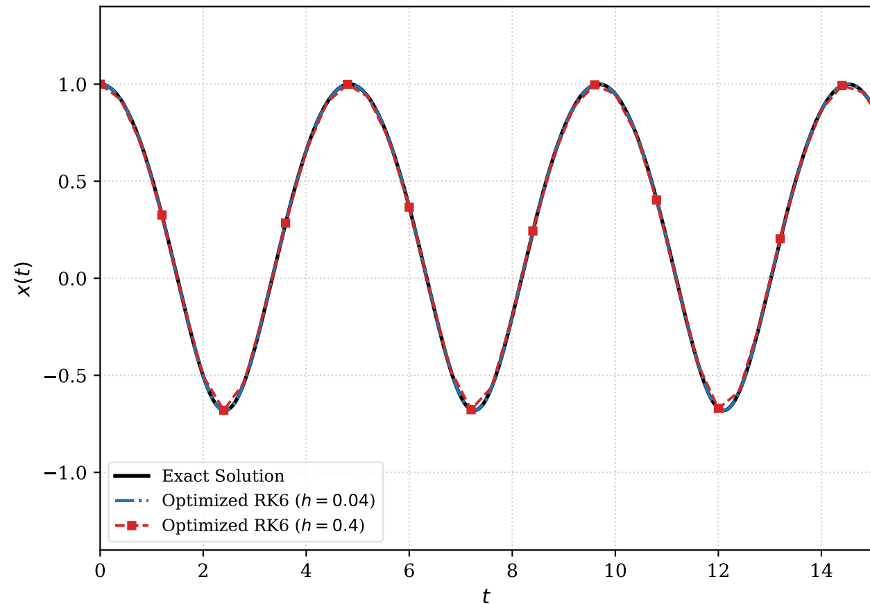
Time Domain: Coordinate x(t) Oscillations
