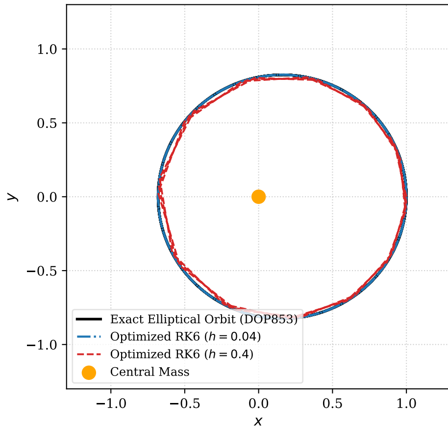
Space Domain: Trajectory Orbit Stability
