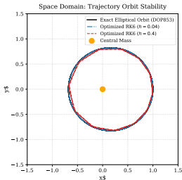
Dynamics of the Gravitational Two-Body Kepler Problem
