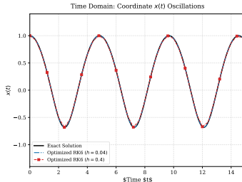
Dynamics of the Gravitational Two-Body Kepler Problem
