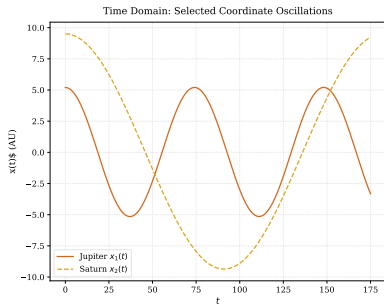
N-Body Outer Planets Simulation
