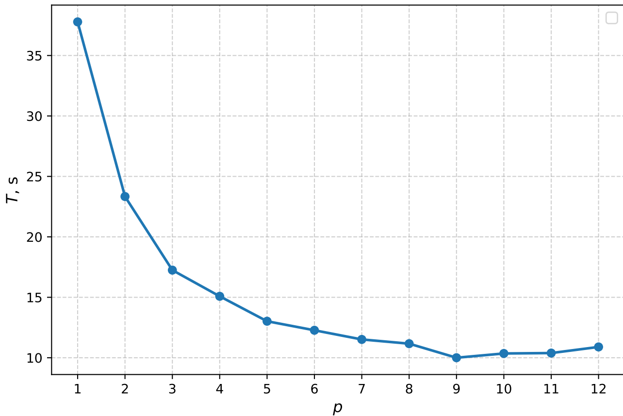
Execution time vs. Process Count
