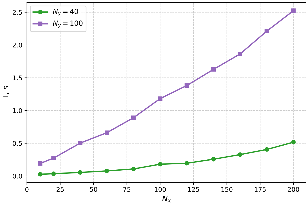
Execution Time vs. Grid Size N_x
