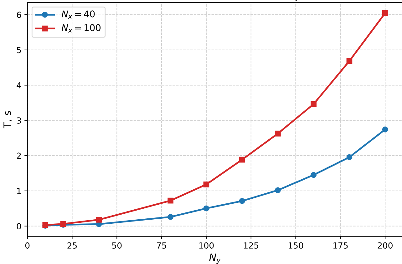
Execution Time vs. Grid Size N_y
