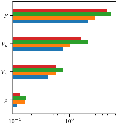
One-Step VRMSE
