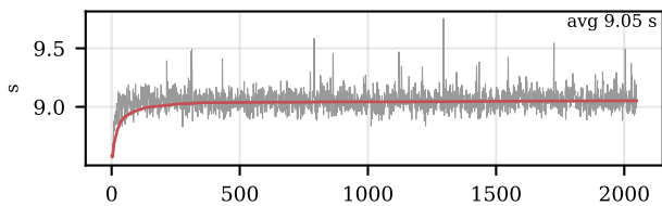
0.84B GPU | recomputation, resident, deferred — time
