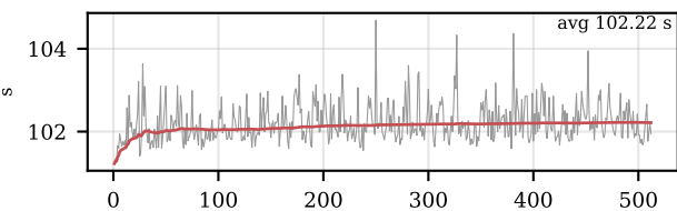
6.9B GPU | recomputation, streamed, in-backward — time
