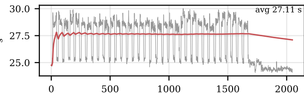
0.84B GPU | recomputation, streamed, deferred (memory floor) — time
