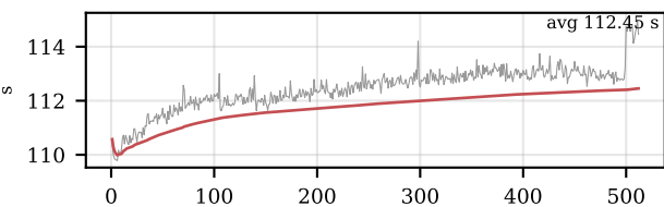
0.84B CPU | recomputation, streamed, deferred — time
