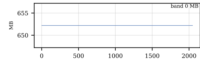
0.84B GPU | recomputation, streamed, deferred (memory floor) — memory
