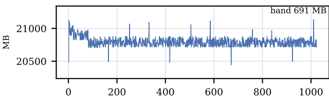
0.84B CPU | retained graph, resident, in-backward — memory
