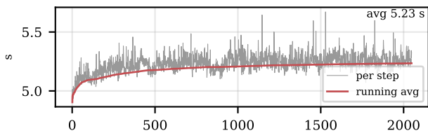
0.84B GPU | retained graph, resident, in-backward (fastest) — time
