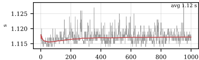
6.9B GPU serving | resident, KV cache — time
