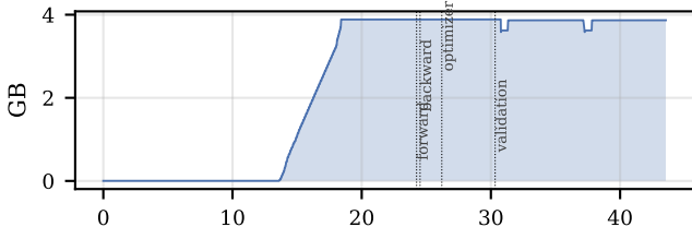
recomputation, streamed, deferred
