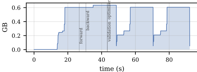
recomp., streamed, in-backward
