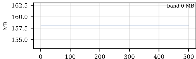
0.84B CPU serving | ONNX runtime, disk-streamed weights — memory
