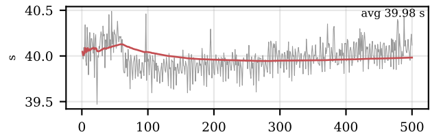
0.84B CPU serving | ONNX runtime, disk-streamed weights — time
