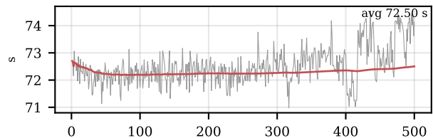
6.9B GPU serving | resident, KV cache — time
