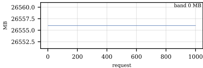
6.9B GPU serving | resident, KV cache — memory
