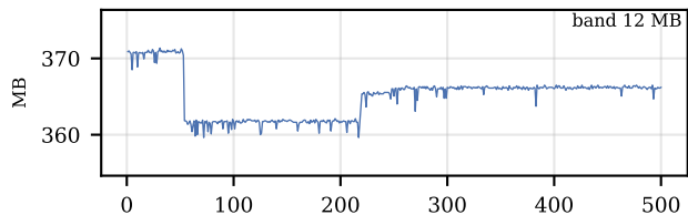
6.9B GPU serving | resident, KV cache — memory
