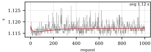
6.9B GPU serving | resident, KV cache — time
