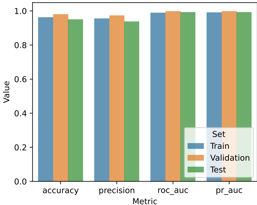
Classification Metrics
