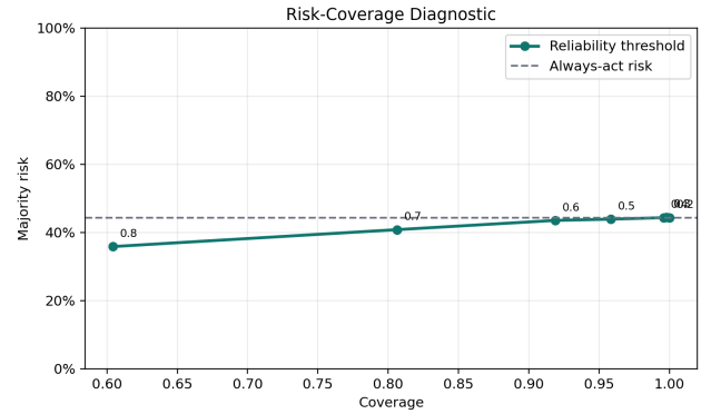
(b) Risk-coverage diagnostic.
