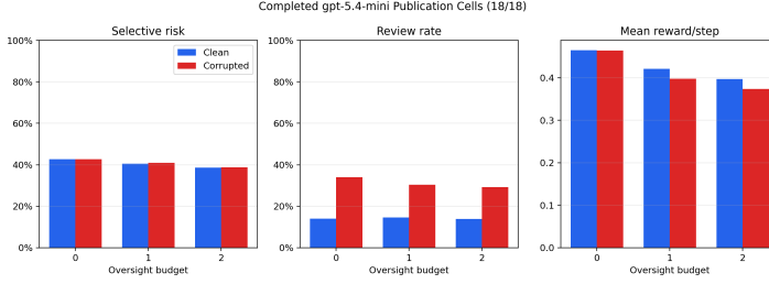
(a) Completed suite budget/corruption grid.
