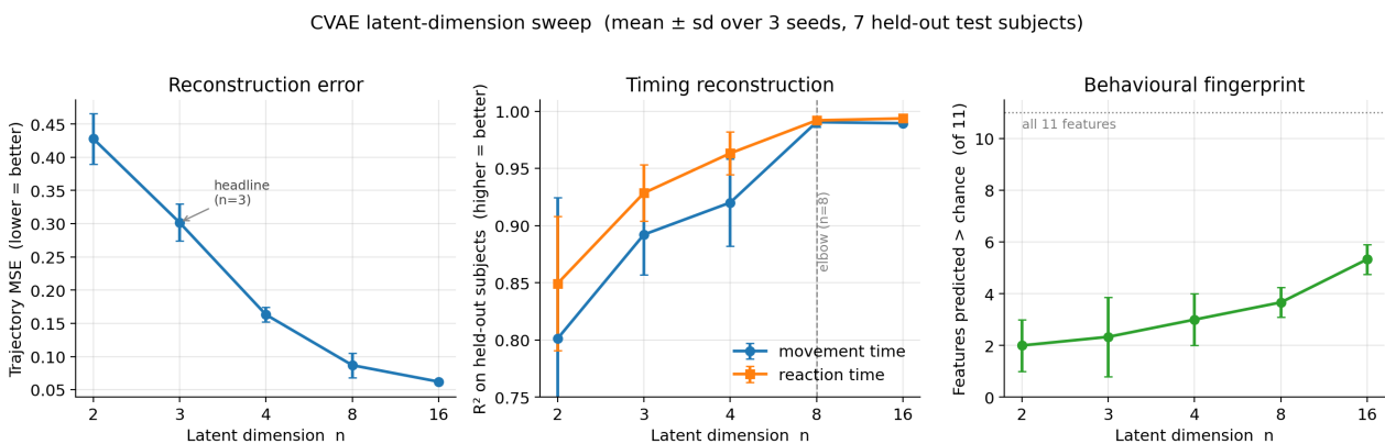
Figure 1. As n grows, reconstruction improves, timing prediction saturates around the n=8 elbow ( R^2 \sim 0.99 ), and the number of behavioural features captured rises.
