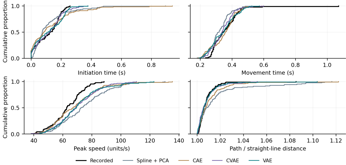
Figure 4. Recorded and generated empirical cumulative distributions for subject01 at n = 8 (fold 2, seed 42). A smaller gap from the black recorded curve indicates closer marginal fidelity. These four features were chosen for distinct meanings, not favorable scores. The cohort analysis includes all eleven features; Appendix A13 shows all curves at both capacities. Differences in this illustrative participant are not separate significance tests.
