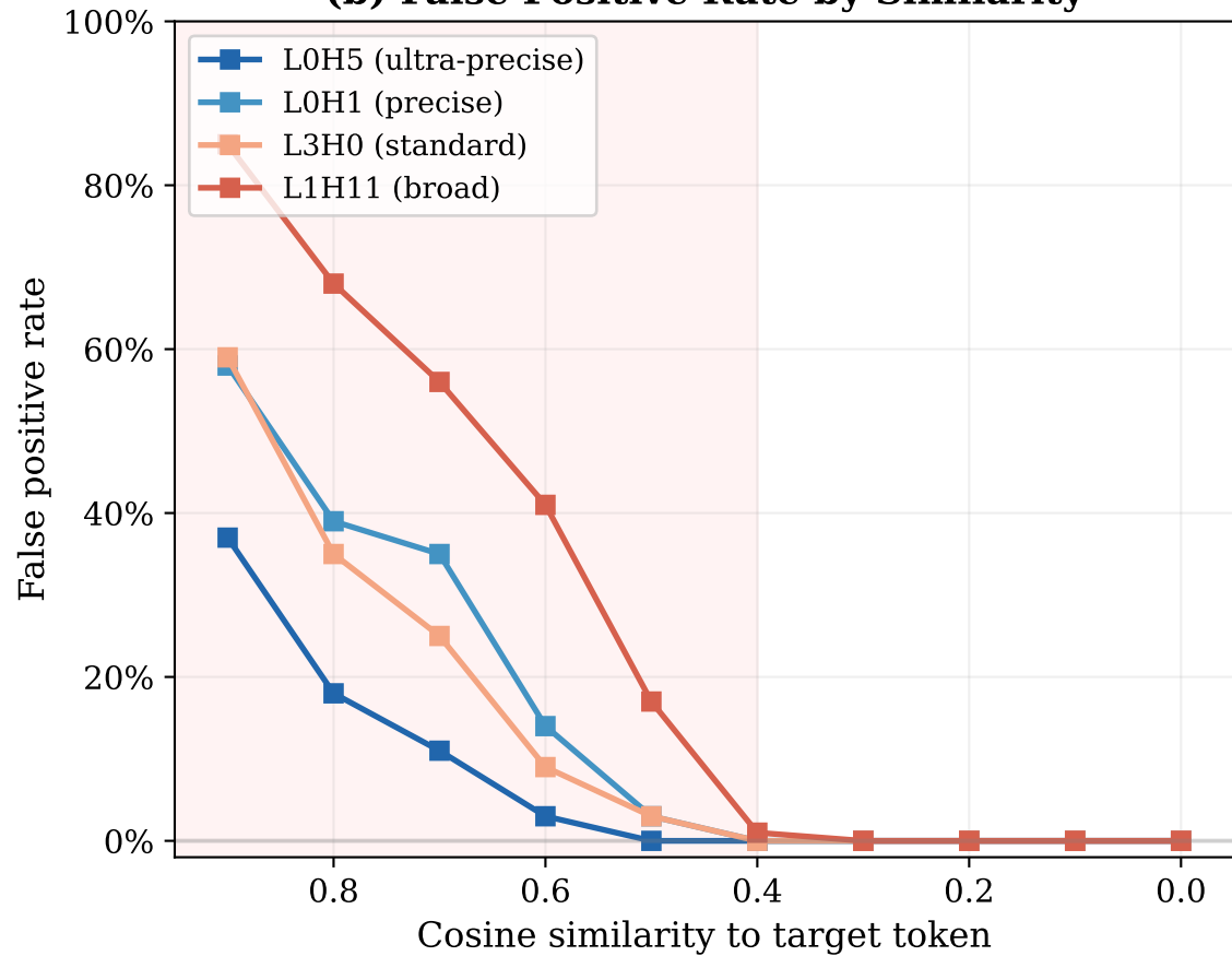
(b) False Positive Rate by Similarity
