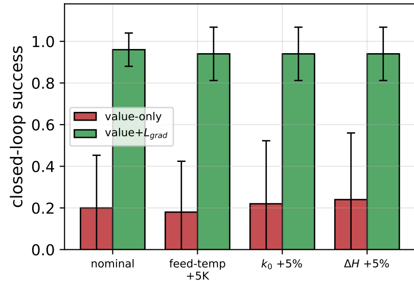
(a) success under plant variation
