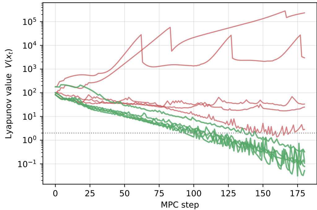
(b) cart-pole
