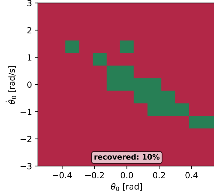
(c) cart-pole — value only
