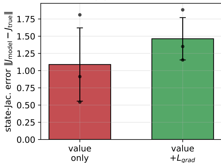
(b) CSTR: error
