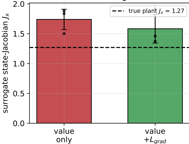
(a) CSTR: magnitude
