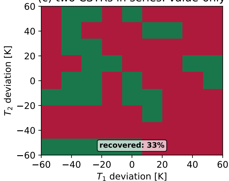
(c) two CSTRs in series: value-only
