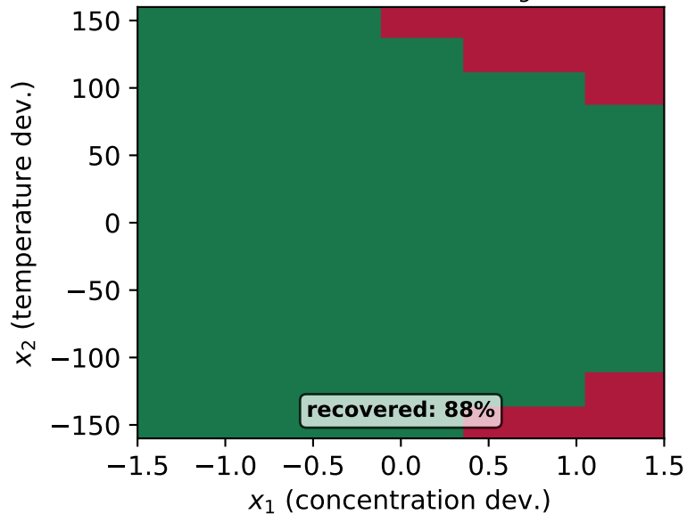
(b) CSTR: value+ L_{grad}
