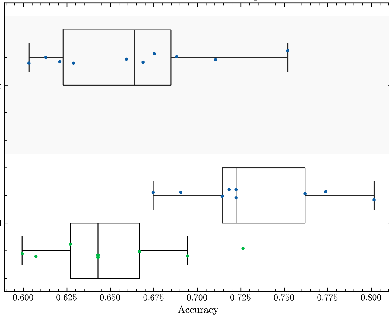
Prediction accuracies for various template estimators
