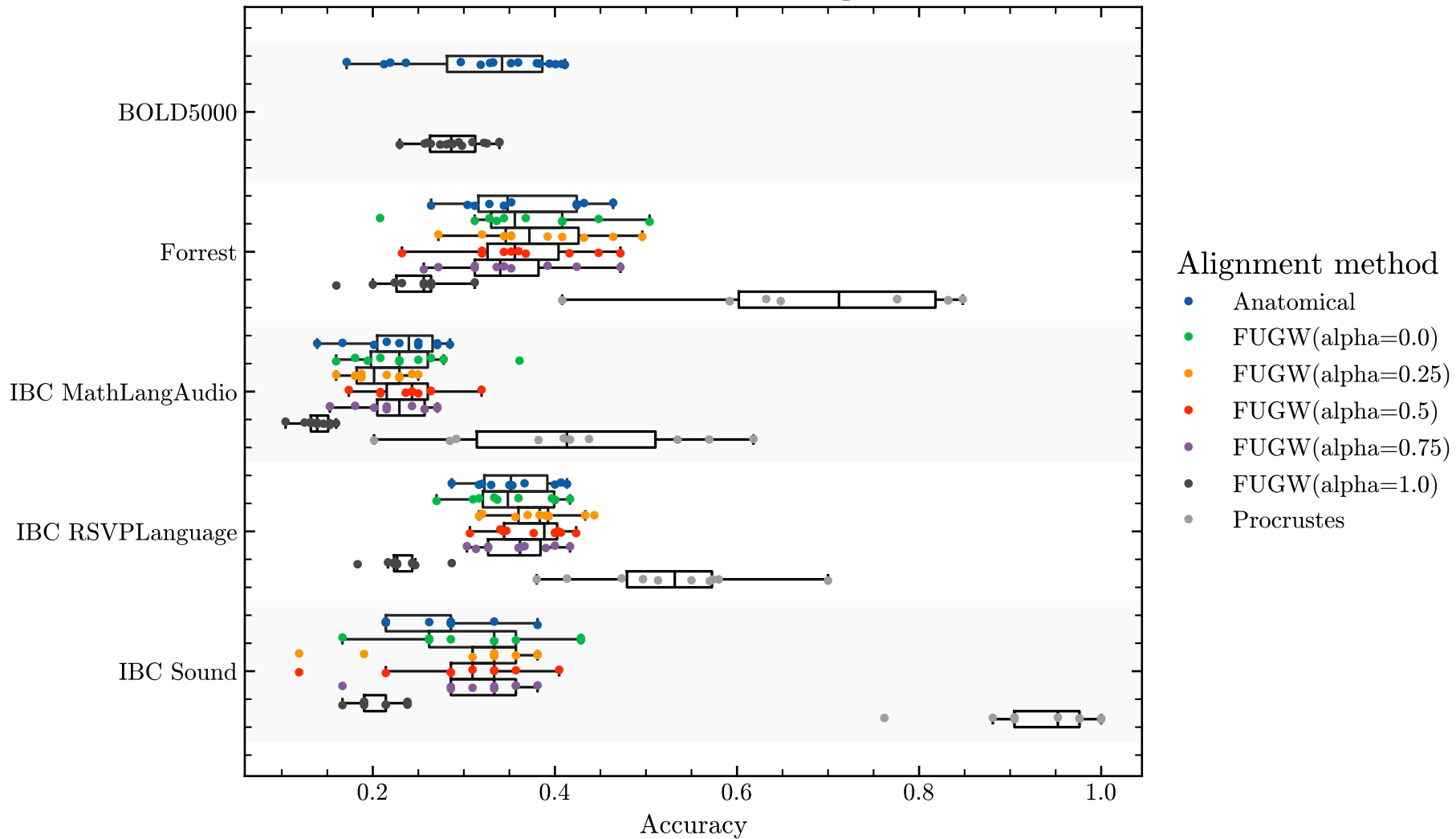
Prediction accuracies for various template estimators
