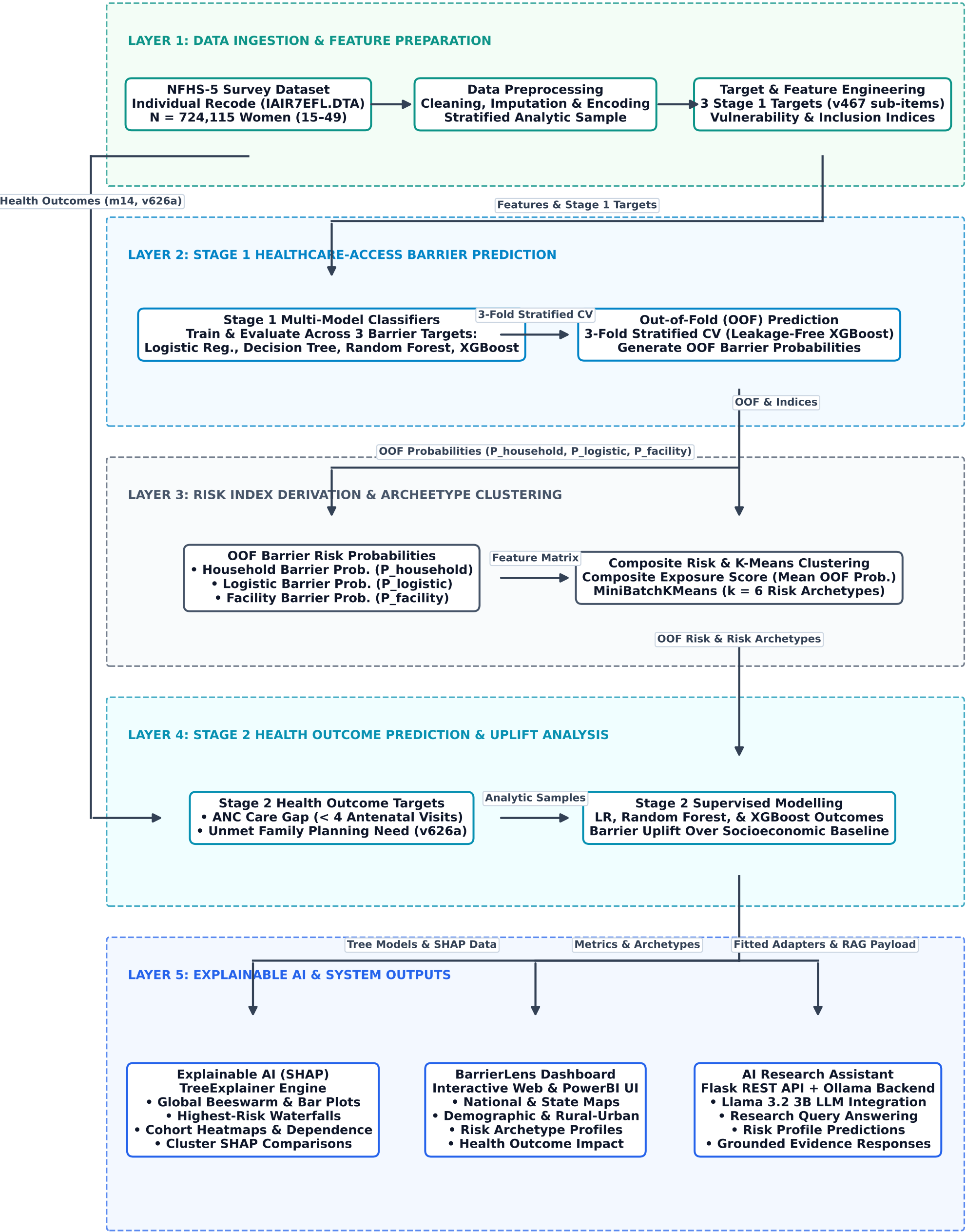
Fig. 5.1. Overall implementation workflow of the BarrierLens system.
